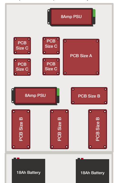
Example 2 - With Optional Battery Box
